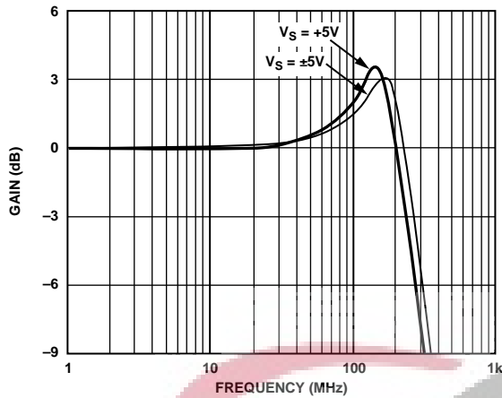
Figure 35. V_{OCM} Frequency Response
